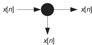
Figure 2.9: Branching operation.
