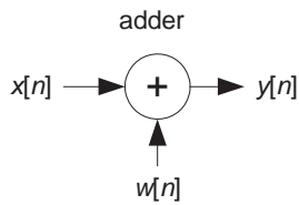
Figure 2.6: Addition operation.
