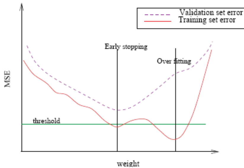
Figure 6.15: Early stopping.
